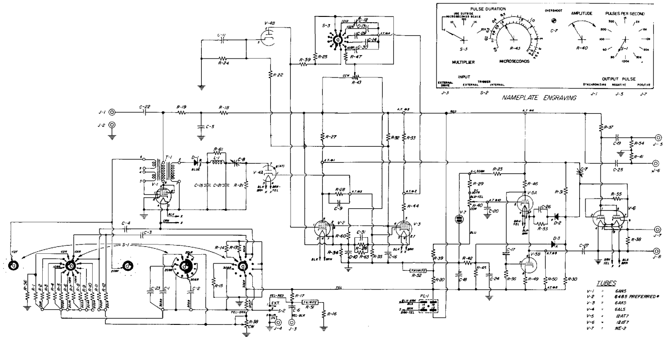
Figure 10. Wiring diagram for the Type 1217-A Unit Pulser.
